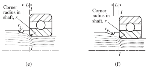
Figure 3.12 Techniques for reducing stress concentration in stepped shaft with bearing: (a) with corner radius only; (b) undercut; (c) inserted ring; (d) undercut to simulate a ring; (e) relief groove; (f) relief groove.
