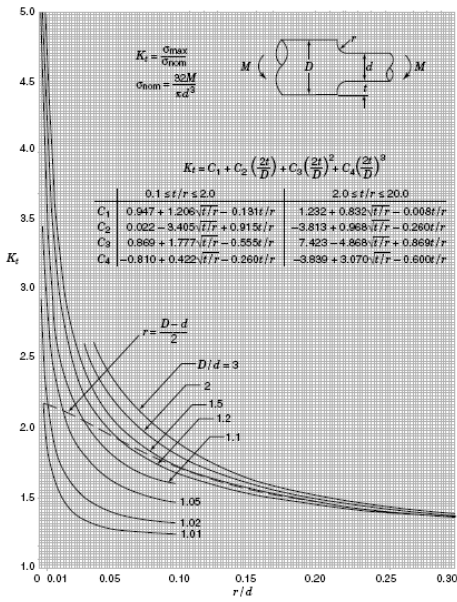
Chart 3.10 Stress concentration factors K_t for bending of a stepped bar of circular cross section with a shoulder fillet (based on photoelastic tests of Leven and Hartman 1951; Wilson and White 1973).
